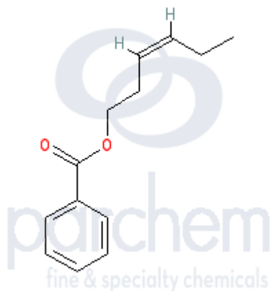
Chemical Structure
